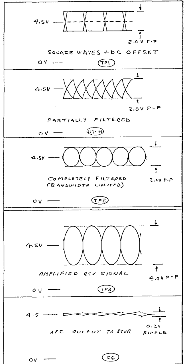
Figure 1. Waveforms at Major Circuit Points
